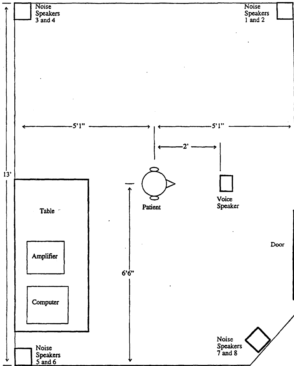
Figure 3: Arrangement of test room.
