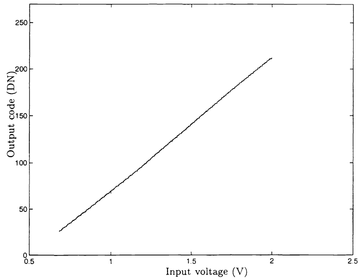
Figure 6. Measured ADC transfer curve.
