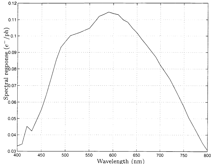
Figure 7. Measured average spectral response of the imager.
