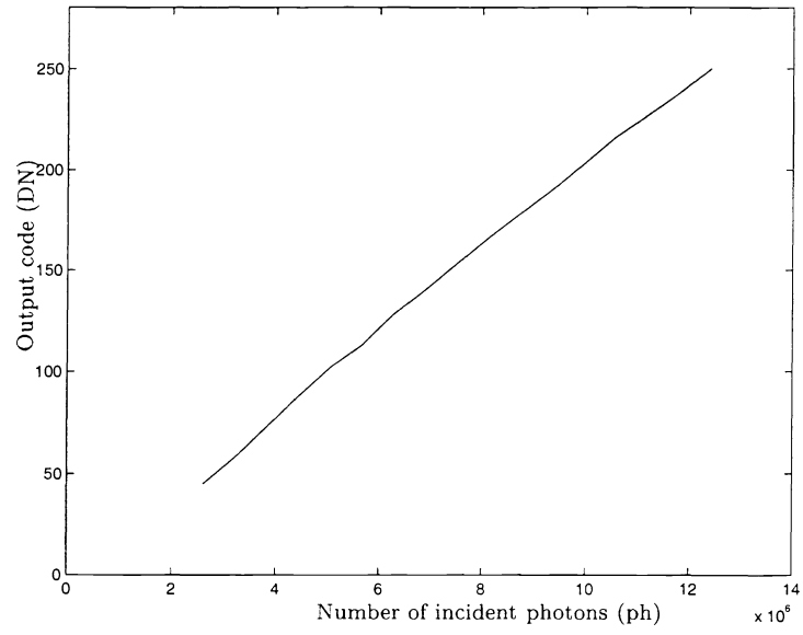
Figure 5. Measured signal transfer curve.
