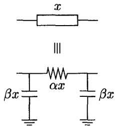
Figure 2: A segment of an interconnect wire with width x is modeled as a conductance \alpha x and two capacitances to the ground \beta x .
