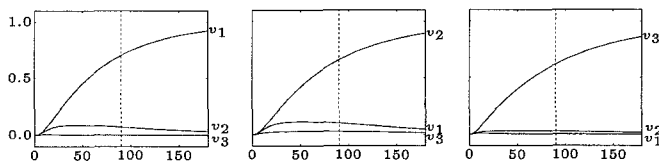
Figure 12: Responses for the solution shown in Figure 11. The voltages at the output nodes, due to a step applied to the first wire (left figure), second wire (center), or third wire (right). The dashed line marks the dominant time constant.
