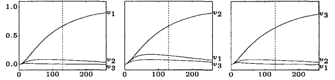
Figure 10: Responses for solution of Figure 9. The voltages at the output nodes due to a step applied to the first wire (left figure), second wire (center), or third wire (right). The dashed line marks the dominant time constant.
