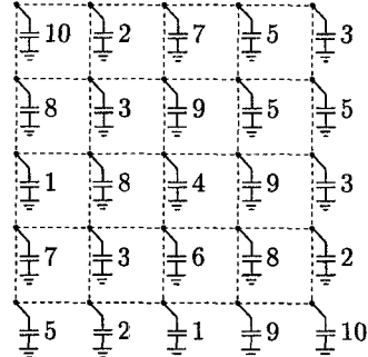
Figure 3: RC mesh example with 4 \times 4 segments, and the numerical values of the load capacitances used in the calculation.
