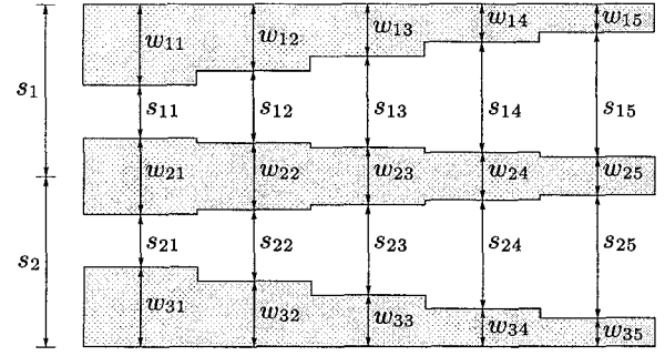
Figure 7: Wire sizing and spacing. Three parallel wires consisting of five segments each. The conductance and capacitance of the j th segment of wire i is proportional to w_{ij} . There is a capacitive coupling between the i th segments of wires 1 and 2, and between the i th segments of wires 2 and 3, and the value of this parasitic capacitance is inversely proportional to s_{1i} , and s_{2i} , respectively. The optimization variables are the 15 segment widths w_{ij} and the distances s_1 and s_2 .
