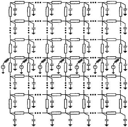
Figure 1: Clock distribution network modeled as an RC mesh. Each rectangular element represents a wire, which we model as a single \pi -segment as in Figure 2. The drivers switch simultaneously. We are interested in the tradeoff between delay (dominant time constant) and total dissipated power. The variables are the widths of the N^2 segments, where N is the number of segments in each column and row.
