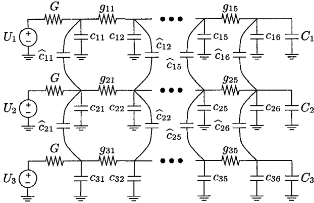
Figure 8: RC model of the three wires shown in Figure 7. The wires are connected to voltage sources with output conductance G at one end, and to load capacitors C_i at the other end. The conductances g_{ij} and capacitances c_{ij} are part of the \pi -models of the wire segments. The capacitances \hat{c}_{ij} model the capacitive coupling. The conductances and capacitances depend on the geometry of Figure 7 in the following way: g_{ij} = \alpha w_{ij} , c_{i1} = \beta w_{i1} , c_{ij} = \beta(w_{ij} + w_{i(j-1)}) ( 1 < j < 6 ), c_{i6} = \beta w_{i5} , \hat{c}_{i1} = \gamma/s_{i1} , \hat{c}_{ij} = \gamma/s_{ij} + \gamma/s_{i(j-1)} ( 1 < j < 6 ), \hat{c}_{i6} = \gamma/s_{i5} .
